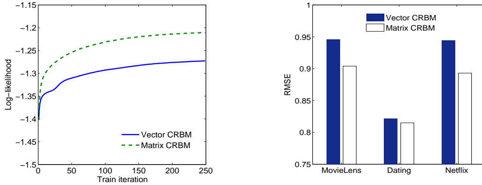
(a) Monitoring pseudo-likelihood in training (b) RMSE on test data
